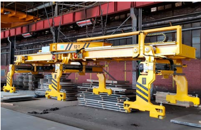
SHEET LIFTER
